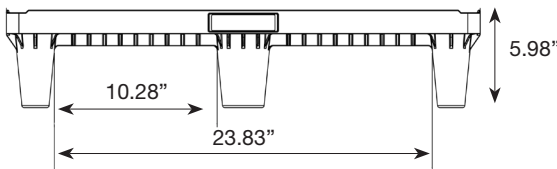
30" side view
