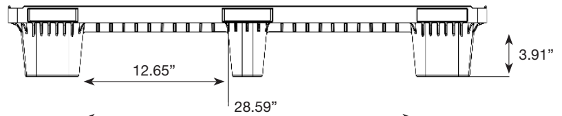
42" side view
